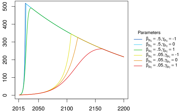
Figure 9: Examples of carbon price paths included in our calibration set
