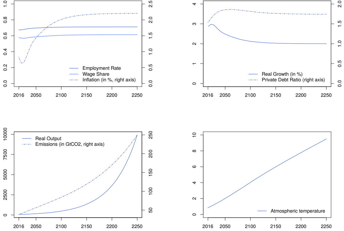
Figure 1: Trajectories of the main simulation variables absent climate change and climate policy.
