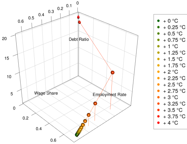
Figure 3: Perturbation of the Solovian steady state parameterized by temperature in the Type 3 scenario.
