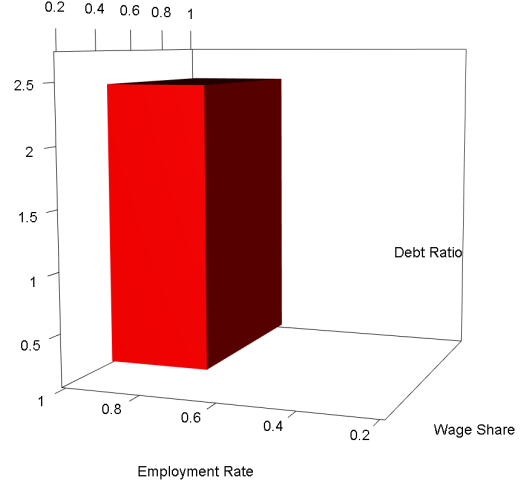
Figure 5: “Good” basin of attraction in the Type 1 scenario.
