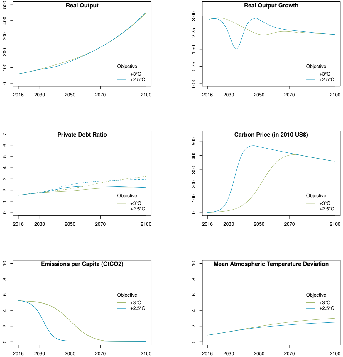
Figure 11: Trajectories for the Type 1 scenario compatible with +2.5^{\circ}\text{C} and +3^{\circ}\text{C} (in dashed curves, the trajectories for the private debt ratio in the Type 3 scenario).
