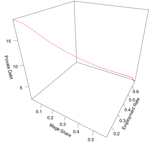
Figure 7: Phase diagram for the Type 3 scenario over the period 2016–2130.
