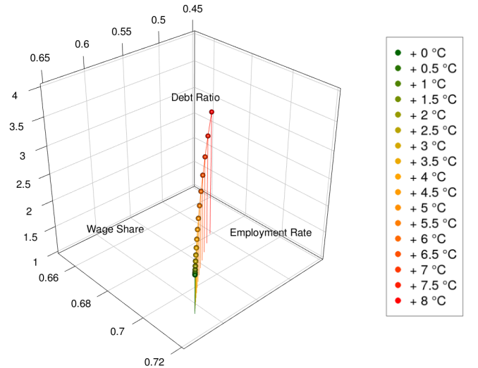
Figure 2: Perturbation of the Solovian steady state parameterized by temperature in the Type 1 scenario.
