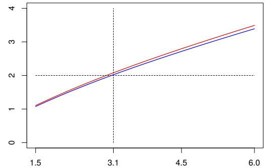
Figure 8: Temperature increase in 2100 as a function of climate sensitivity whenever zero net emission is reached in 2016 (blue line) or 2018 (red line)
