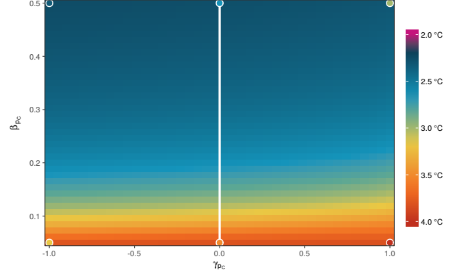
Figure 10: Heatmap depending on the carbon price path in the Type 3 scenario with ECS=3.1.
