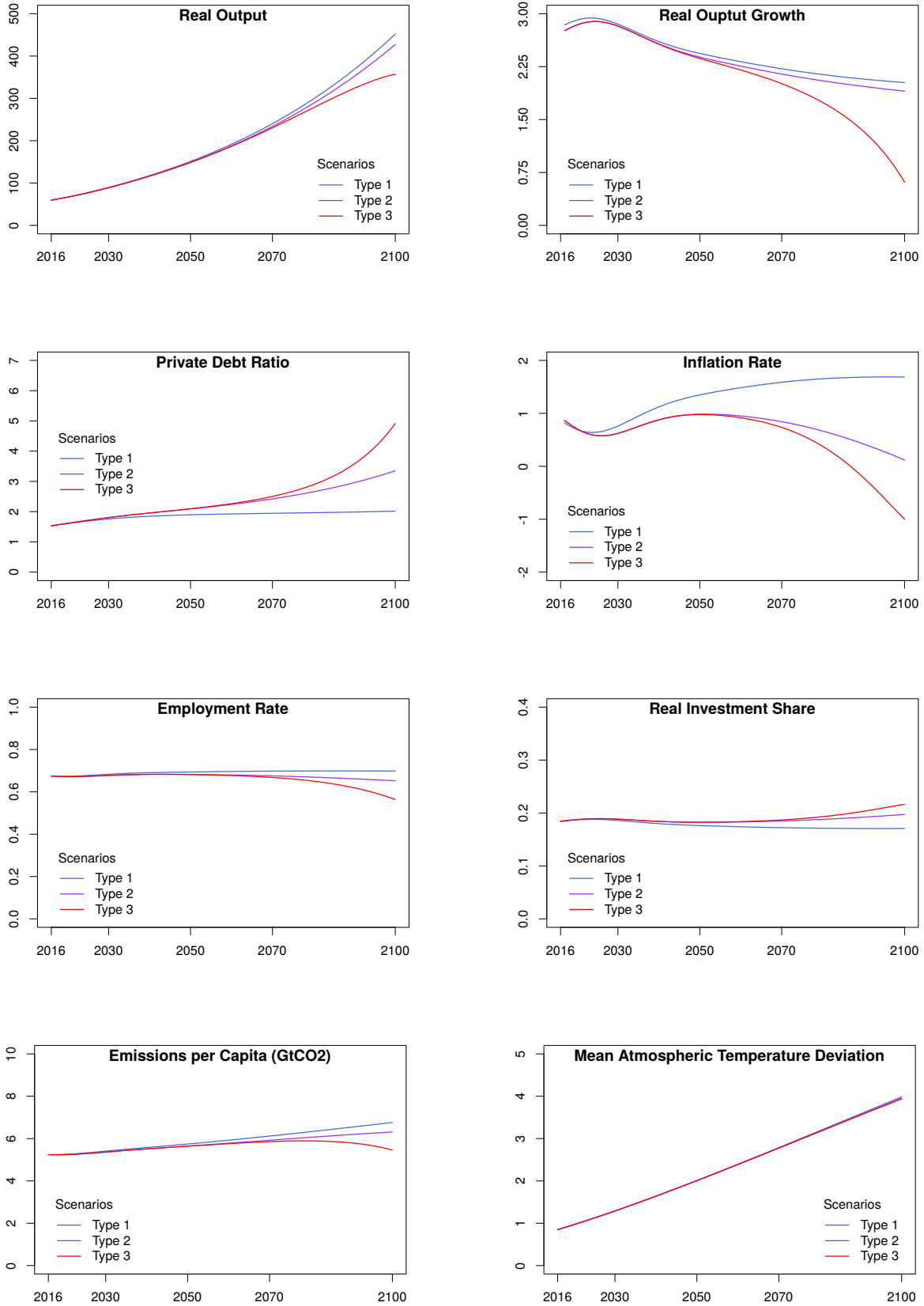
Figure 6: Macroeconomic trajectories without proactive public policies.
