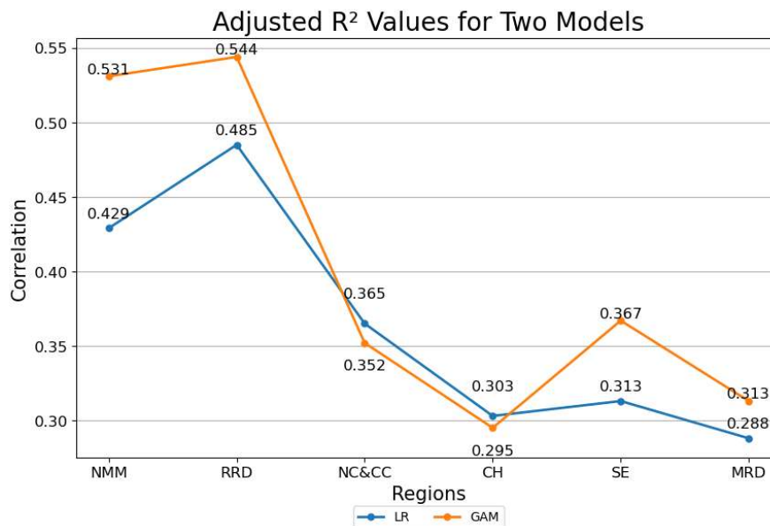
Figure 7: Adjusted R^2 Values for Two Models
